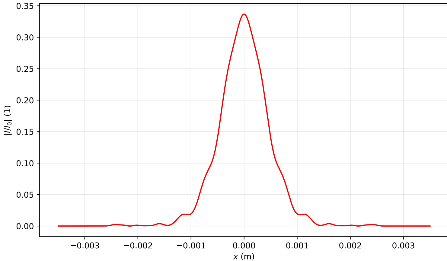
Intensity profile I(x, y = 0, z = 2.866)/I_0 , P_{in}=1.0P_{cr} , artificial time
